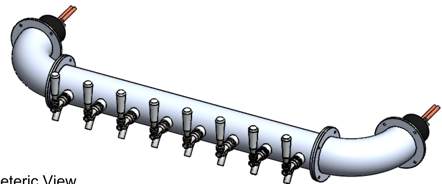
Isometric View (For reference purpose only)
